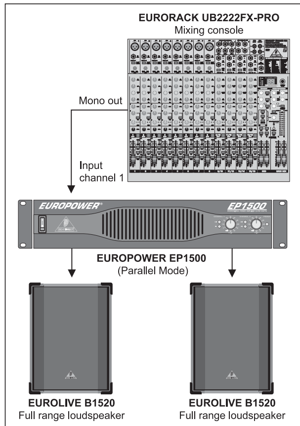
Fig. 3.3: Parallel operation
